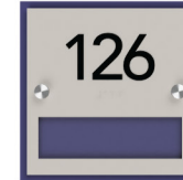
Room Number B 6" x 6" • Name insert slot (1.25" x 4.5") • Stainless steel caps • 1/32" Raised text • Grade 2 braille
