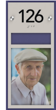
Room Number C 6" x 13" • Photo insert slot (5" x 7") • Name insert slot (1.25" x 4.5") • Stainless steel caps • 1/32" Raised text • Grade 2 braille
